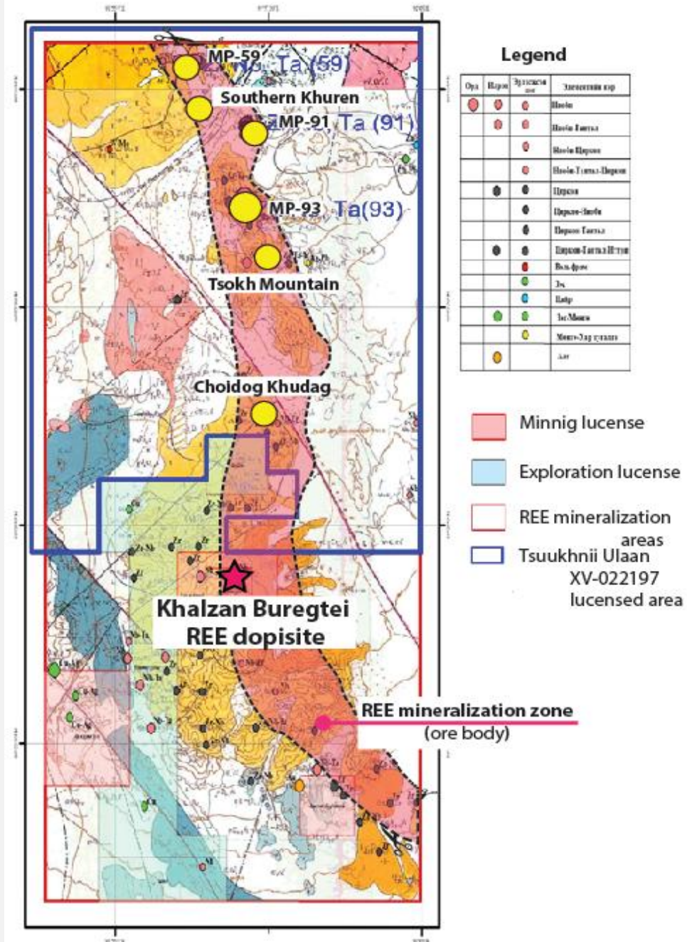
Geological and mineralization map scale by 1:100 000
